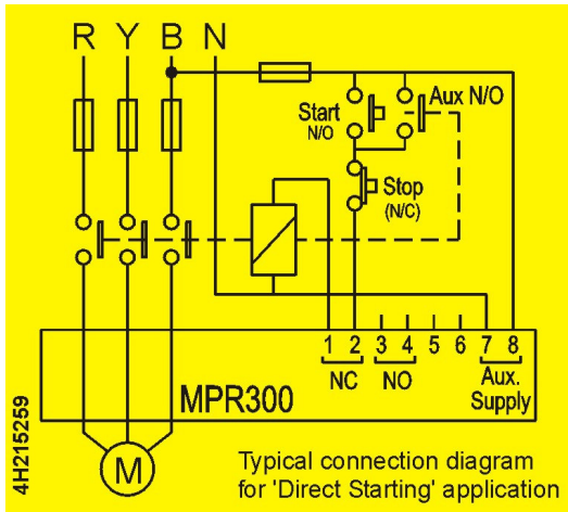
Fig-1a Wiring diagram for MPR300 (NORMAL MODE)
